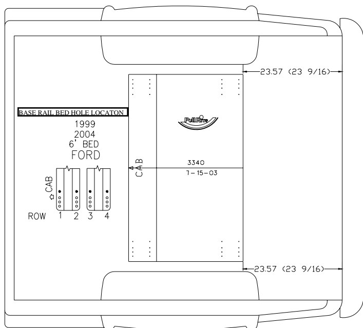
TEMPLATE METHOD
