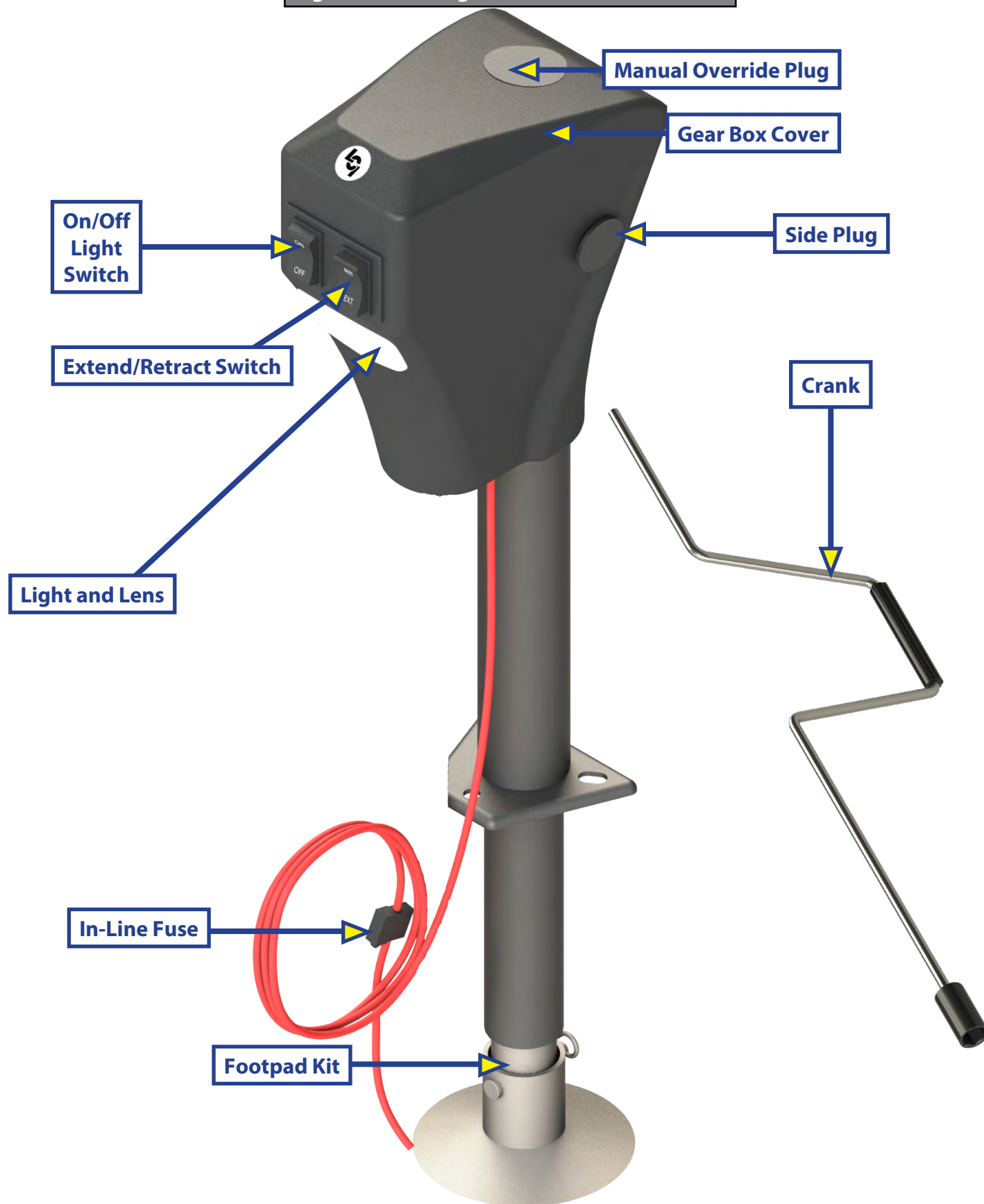
Fig. 1 Power Tongue Jack Kit - Part #285318
